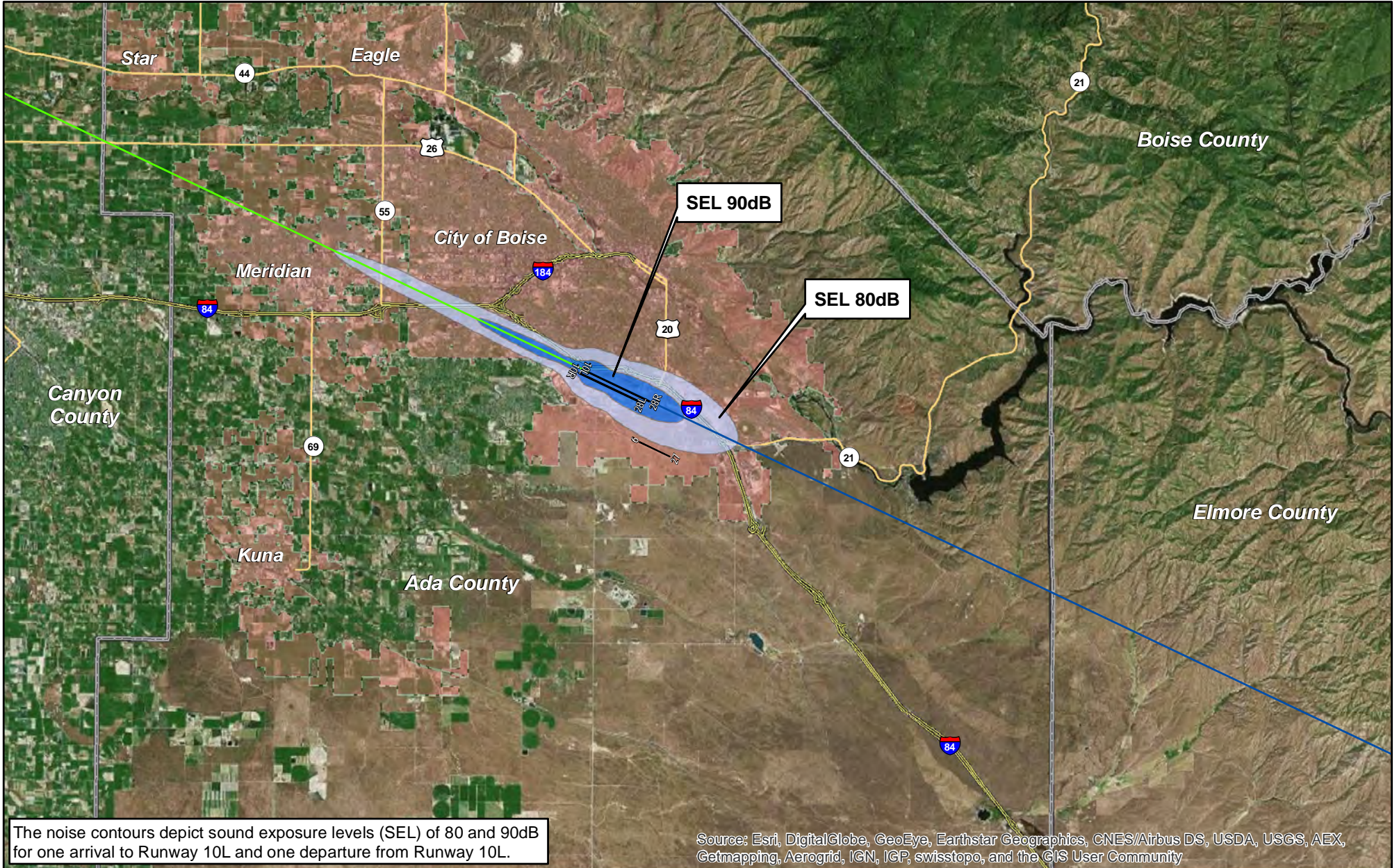
Figure B-16 A-10A Sound Exposure Level (80dB/90dB) Noise Contour
